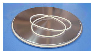
Lid, 'O' Ring Seal and Clampband supplied as standard
